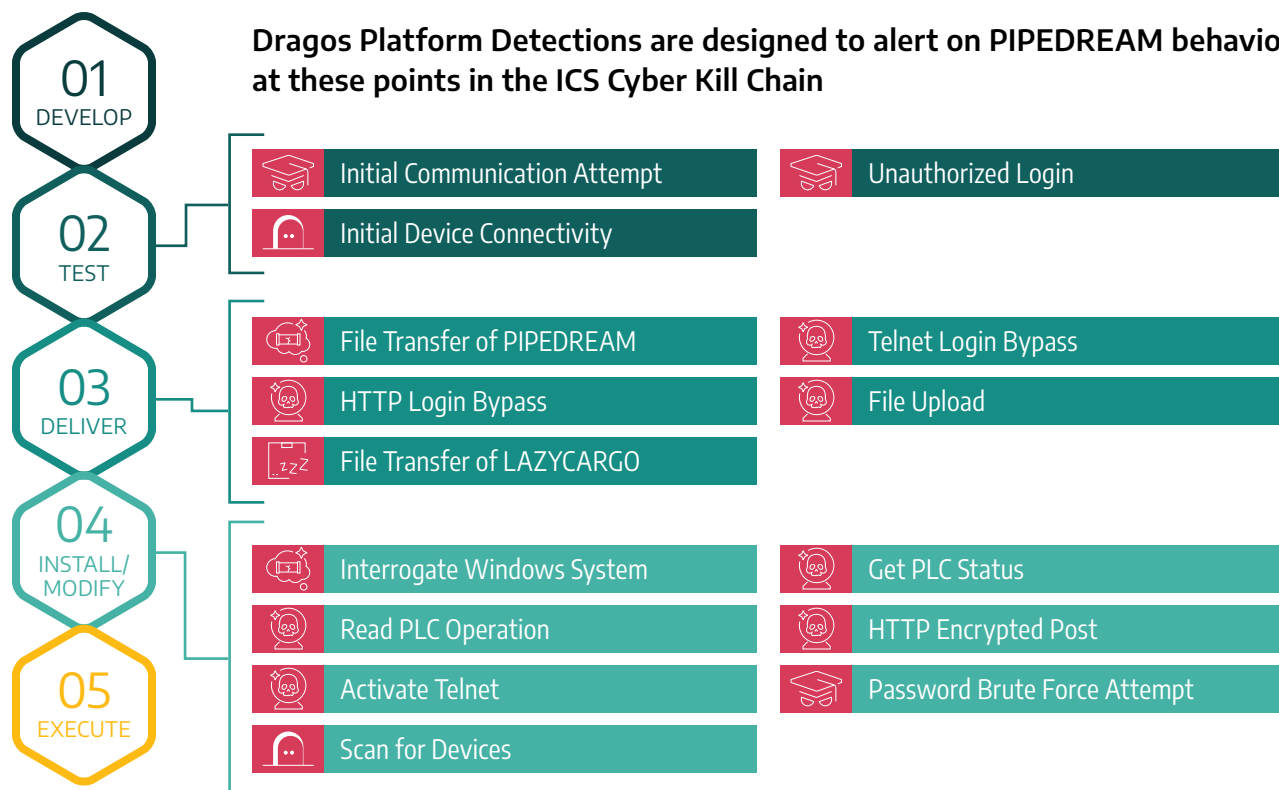
Figure 3: ICS Cyber Kill Chain
